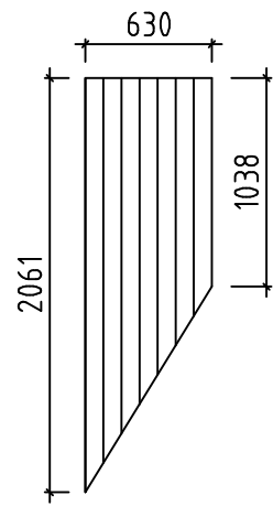
Shield 1 / 2tk
